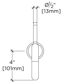
FRONT VIEW SCALE: 1\frac{1}{2}"=1'-0"
