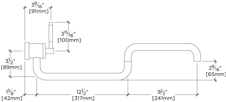
SIDE VIEW SCALE: 1\frac{1}{2}"=1'-0"
