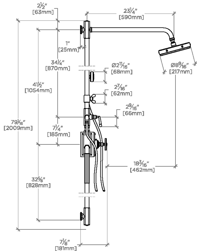
SIDE VIEW
