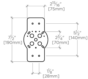
MOUNTING PLATE
