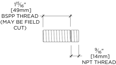
ADAPTER INCLUDED - INTERNATIONAL USE ONLY NOT TO SCALE
