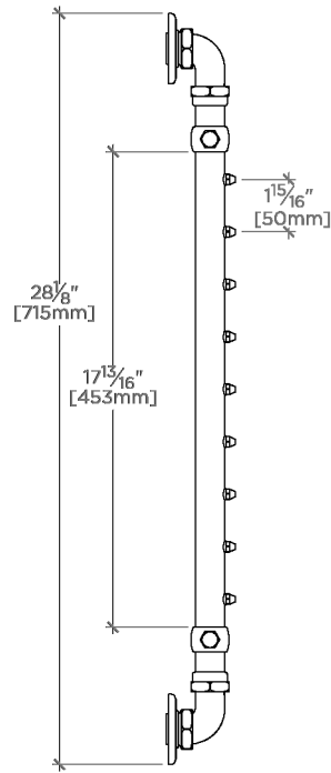
SIDE VIEW SCALE: 1\frac{1}{2}"=1'-0"
