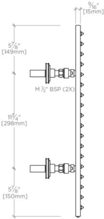
SIDE VIEW SCALE: 1 1/2"=1'-0"
