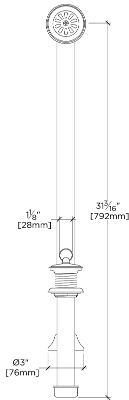
FRONT VIEW SCALE: 1 1/2"=1'-0"
