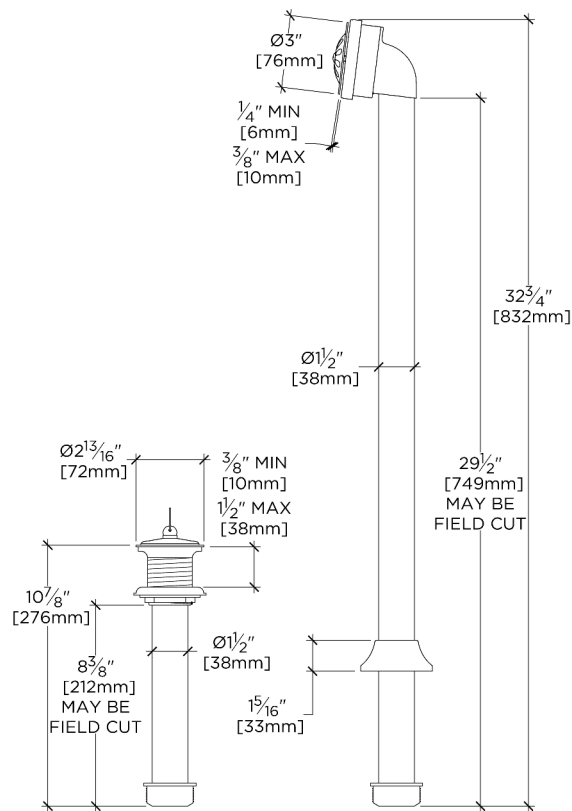
SIDE VIEW SCALE: 1 1/2"=1'-0"
