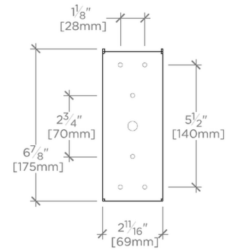
MOUNTING PLATE SCALE: 2"=1'-0"
