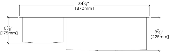
FRONT VIEW SCALE: 1"=1'-0"
