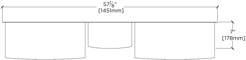
FRONT VIEW
