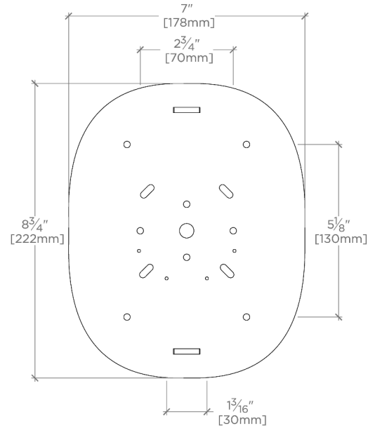
MOUNTING PLATE
