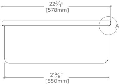
FRONT VIEW SCALE: 1"=1'-0"
