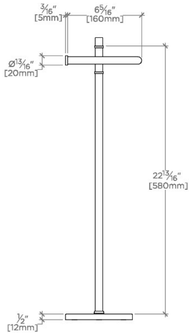
FRONT VIEW SCALE: 1\frac{1}{2}"=1'-0"
