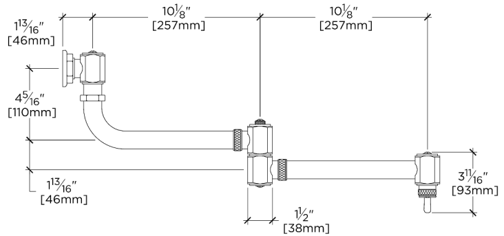
SIDE VIEW SCALE: 1 1/2"=1'-0"
