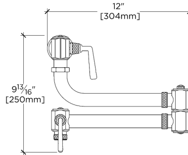
FOLDED VIEW SCALE: 1 1/2"=1'-0"
