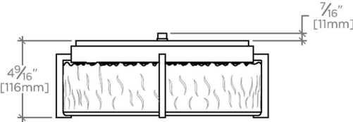
SIDE VIEW SCALE: 1 1/2"=1'-0"
