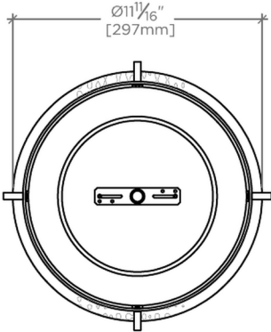
CEILING VIEW SCALE: 1 1/2"=1'-0"
