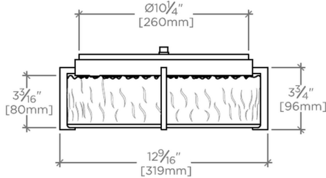
FRONT VIEW SCALE: 1 1/2"=1'-0"
