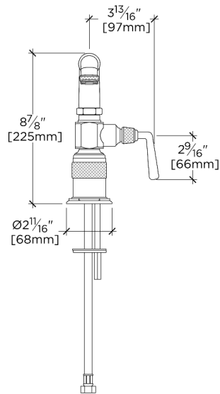
FRONT VIEW SCALE: 1 1/2"=1'-0"
