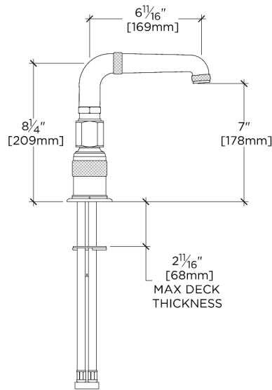
SIDE VIEW SCALE: 1 1/2"=1'-0"
