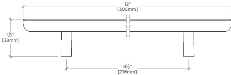
FRONT VIEW
