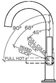
HANDLE OPERATION SCALE: 1 1/2"=1'-0"
