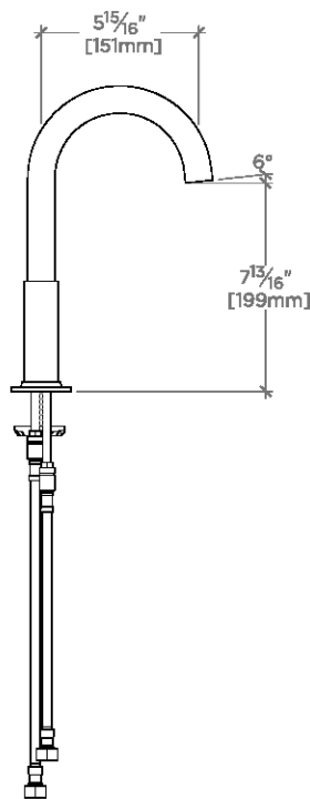
SIDE VIEW SCALE: 1 1/2"=1'-0"
