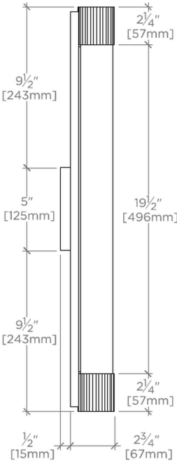
SIDE VIEW SCALE: 1 1/2"=1'-0"
