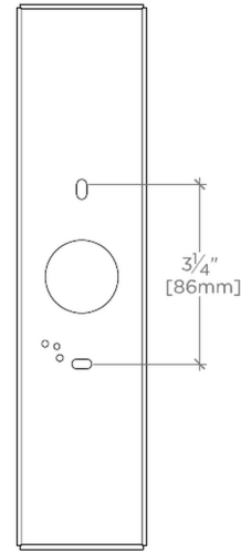
MOUNTING PLATE
