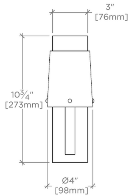
FRONT VIEW SCALE: 1 1/2"=1'-0"
