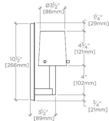
SIDE VIEW SCALE: 1 1/2"=1'-0"
