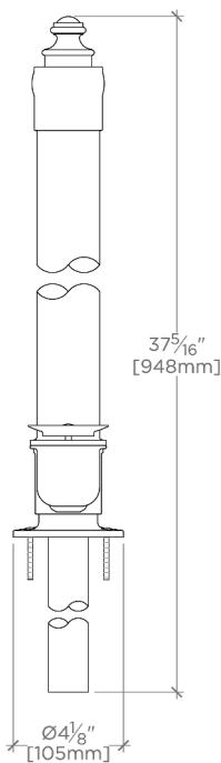
FRONT VIEW SCALE: 1 1/2"=1'-0"
