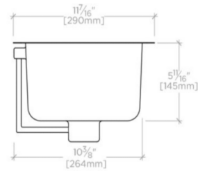
SIDE VIEW SCALE: 1/2"=1'-0"
