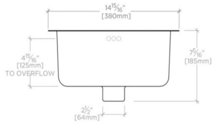
FRONT VIEW SCALE: 1/2"=1'-0"
