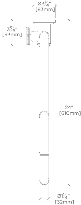
TOP VIEW
