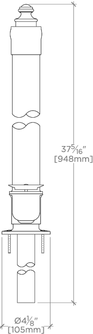
FRONT VIEW SCALE: 1 1/2"=1'-0"
