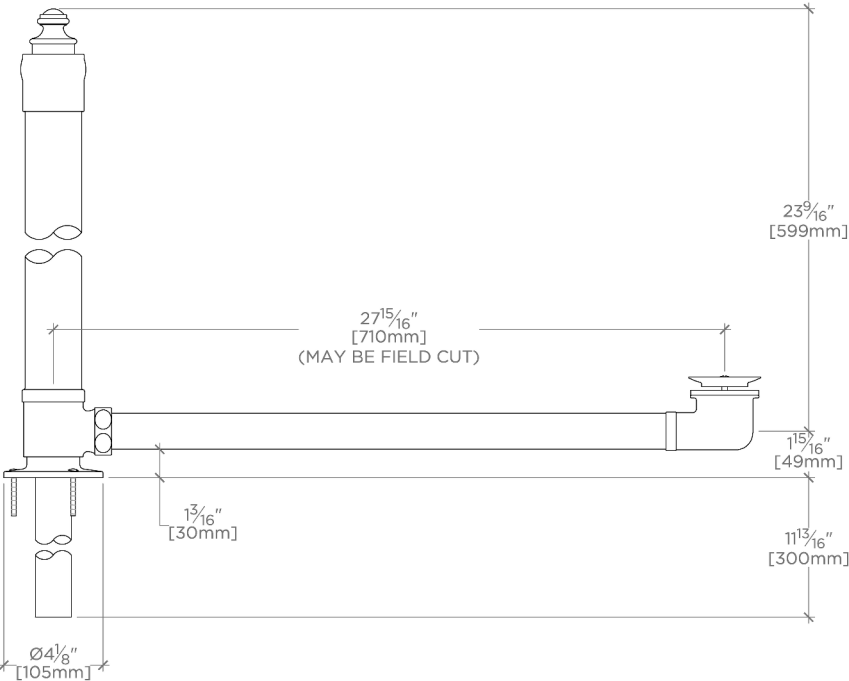
SIDE VIEW SCALE: 1 1/2"=1'-0"
