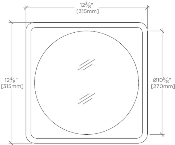
CEILING VIEW
