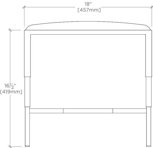
FRONT VIEW SCALE: 1-1/2"=1'-0"
