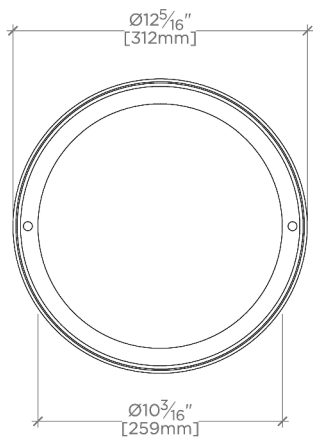
CEILING VIEW SCALE: 1 1/2"=1'-0"
