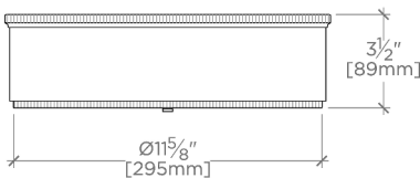
SIDE VIEW SCALE: 1 1/2"=1'-0"
