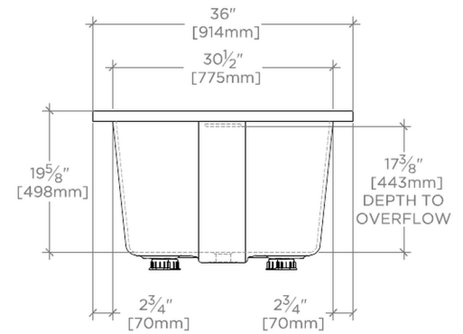
END VIEW
