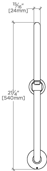
FRONT VIEW SCALE: 1 1/2"=1'-0"
