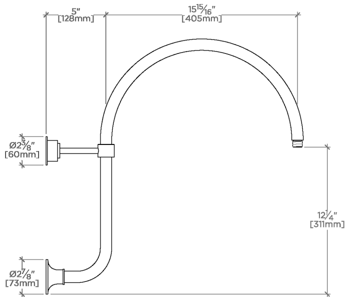
SIDE VIEW SCALE: 1 1/2"=1'-0"
