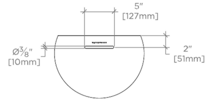
OVERFLOW DETAIL
