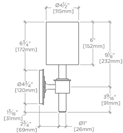
SIDE VIEW SCALE: 1/2"=1'-0"
