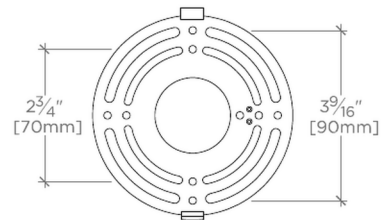
MOUNTING PLATE
