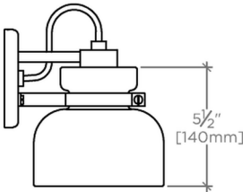
SIDE VIEW SCALE: \frac{1}{2}"=1'-0"
