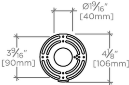
MOUNTING PLATE SCALE: \frac{1}{2}"=1'-0"
