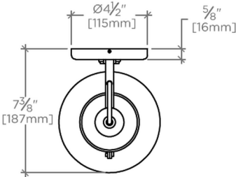
TOP VIEW SCALE: \frac{1}{2}"=1'-0"
