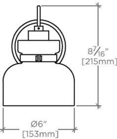
FRONT VIEW SCALE: \frac{1}{2}"=1'-0"
