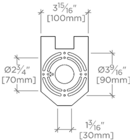
MOUNTING PLATE SCALE: 1 1/2"=1'-0"
