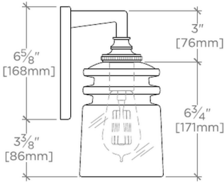
SIDE VIEW SCALE: 1 1/2"=1'-0"
