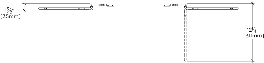
TOP VIEW
