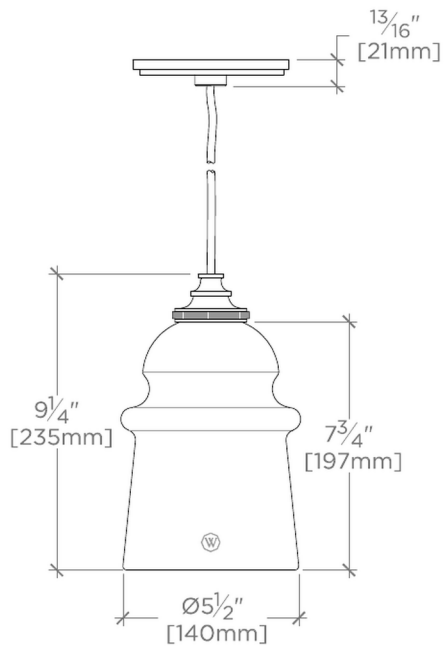
FRONT VIEW SCALE: 2"=1'-0"
