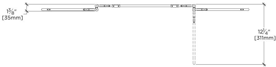
TOP VIEW
