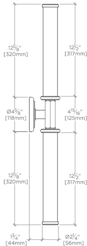
SIDE VIEW SCALE: 1 1/2"=1'-0"
