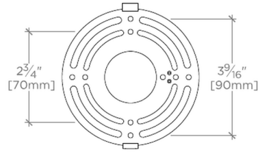
MOUNTING PLATE SCALE: 1 1/2"=1'-0"
