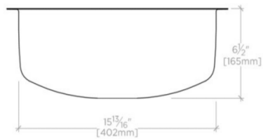
SIDE VIEW SCALE: 1 1/2"=1'-0"
