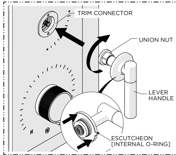
22. CAREFULLY slide the ESCUTCHEON up the LEVER HANDLE to expose the UNION NUT then thread the NUT into the TRIM CONNECTOR until snug.
