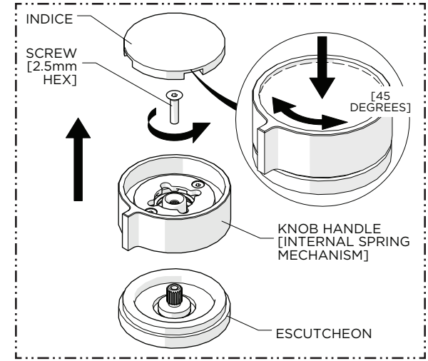
20. Remove the INDICE, center SCREW and KNOB HANDLE from the ESCUTCHEON. Do NOT remove the internal SPRING.
