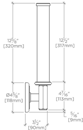
SIDE VIEW SCALE: 1 1/2"=1'-0"
