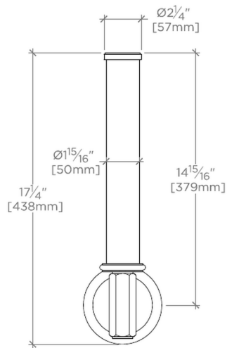
FRONT VIEW SCALE: 1 1/2"=1'-0"
