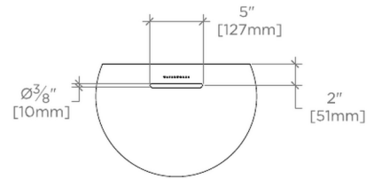
OVERFLOW DETAIL
