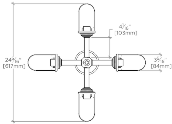
CEILING VIEW
