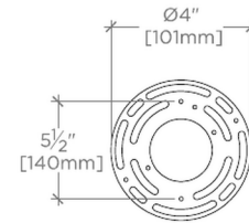
MOUNTING PLATE
