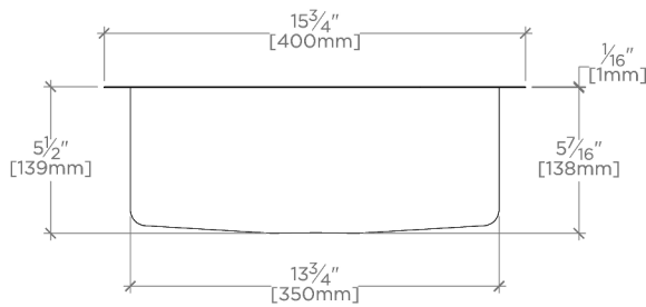
FRONT VIEW SCALE: 1/2"=1'-0"
