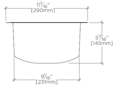
SIDE VIEW SCALE: 1/2"=1'-0"
