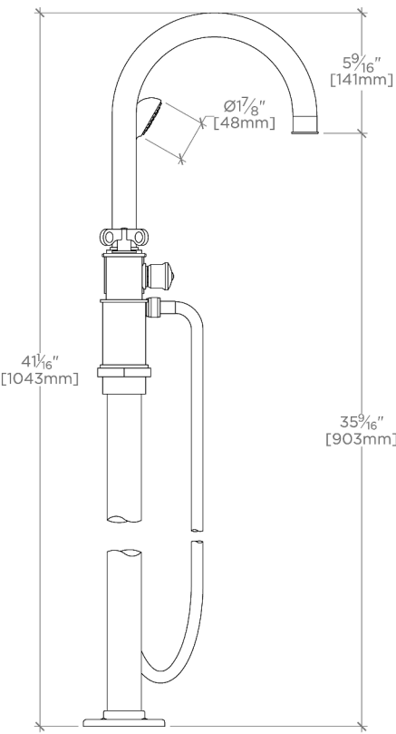
SIDE VIEW SCALE: 1 1/2"=1'-0"
