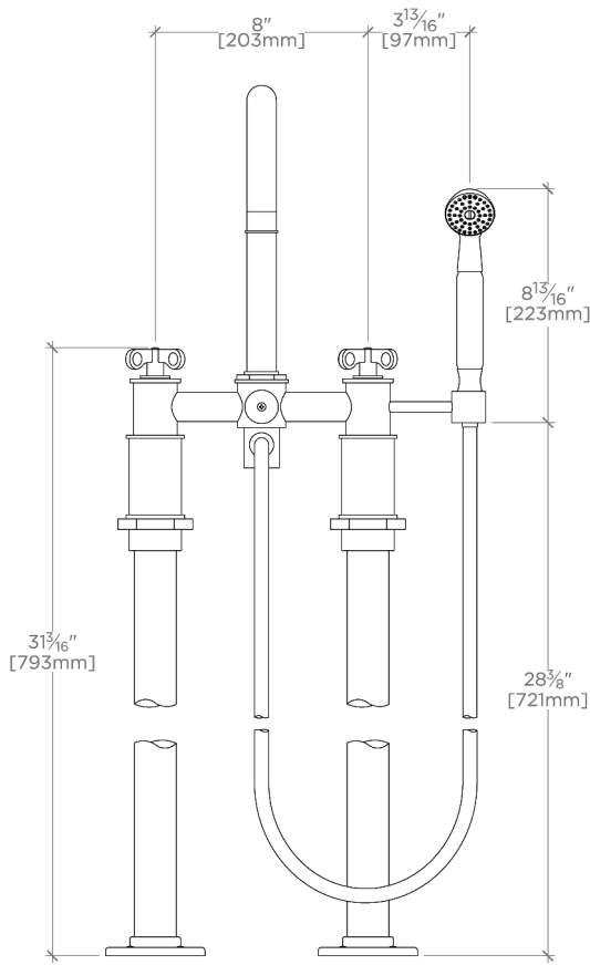
FRONT VIEW SCALE: 1 1/2"=1'-0"
