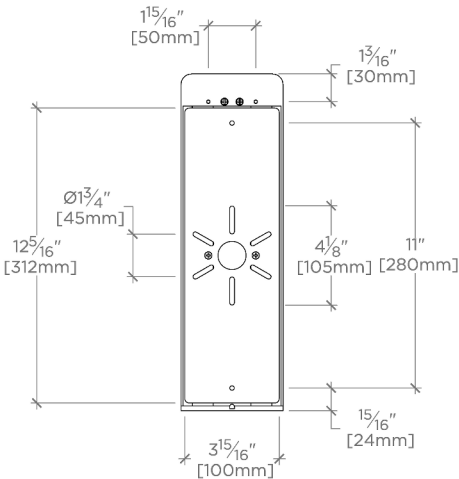
MOUNTING PLATE SCALE: 1 1/2"=1'-0"
