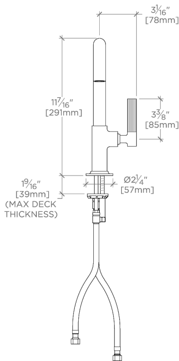
FRONT VIEW SCALE: 1 1/2"=1'-0"
