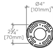
MOUNTING PLATE
