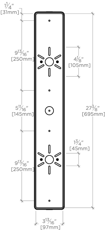
MOUNTING PLATE SCALE: 1 1/2"=1'-0"
