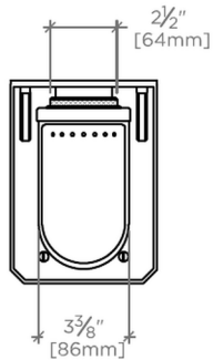
FRONT VIEW SCALE: 1 1/2"=1'-0"
