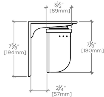
SIDE VIEW SCALE: 1 1/2"=1'-0"
